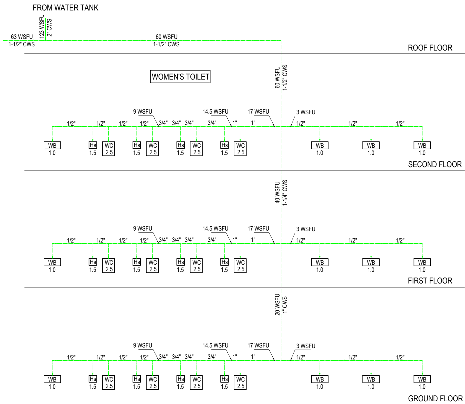
SCHMATIC RISER DIAGRAM COLD WATER SUPPLY (CWS) SYSTEM
